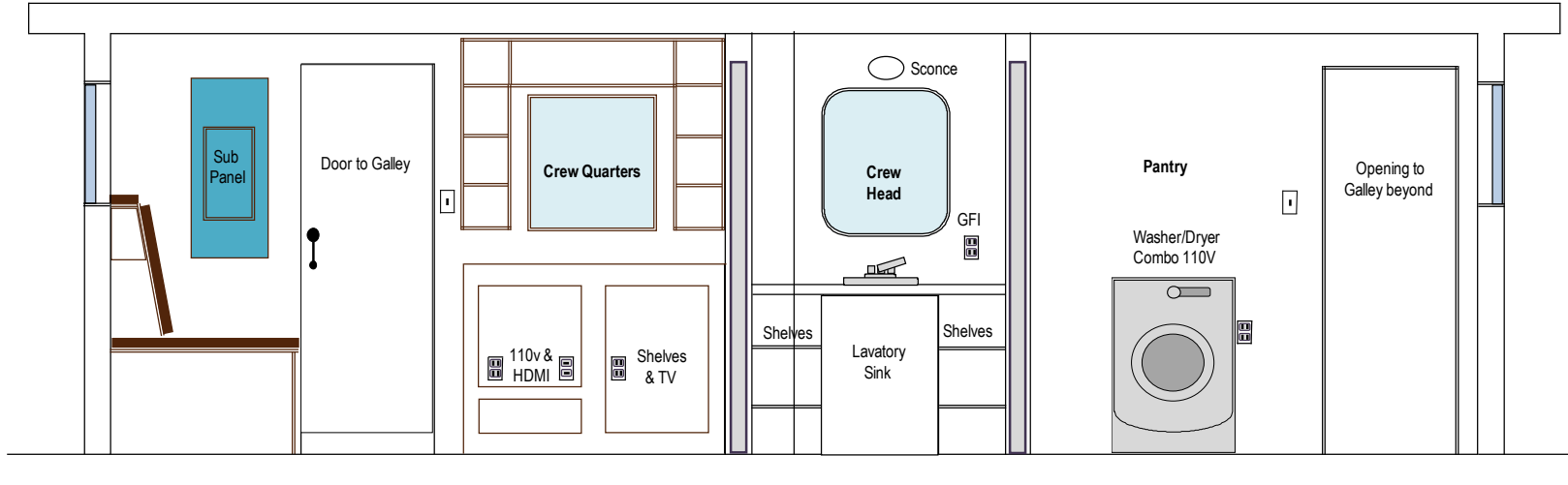
Main Deck Plans Pantry Head & Crew Qtrs Elevation Looking Fore 31209a -GRC-
