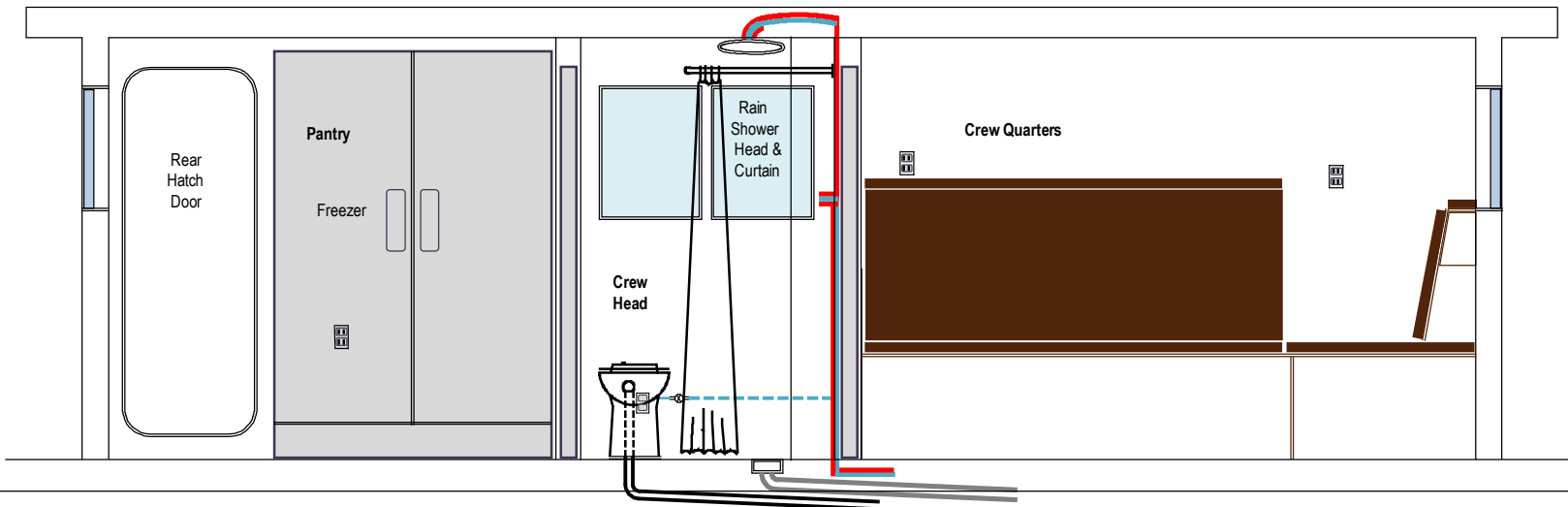
Main Deck Plans Pantry Head & Crew Qtrs Elevation Looking Aft 31209a -GRC-
