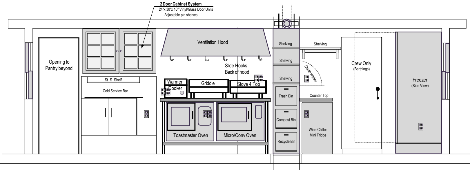
Main Deck Plans Galley Elevation Looking Aft
