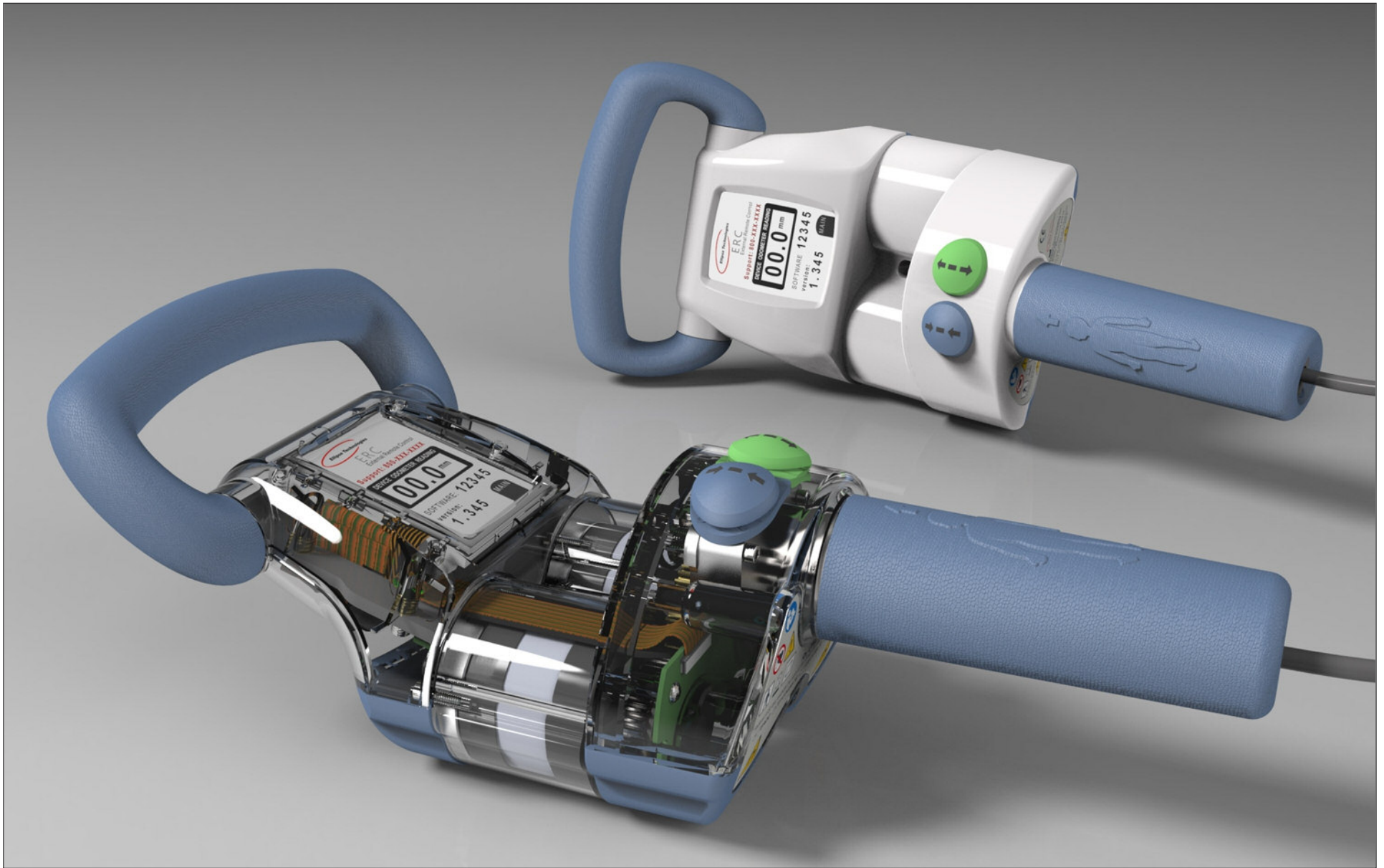
KeyShot rendering of Ellipse Technologies', Magec™ external remote controller, (ERC2).
