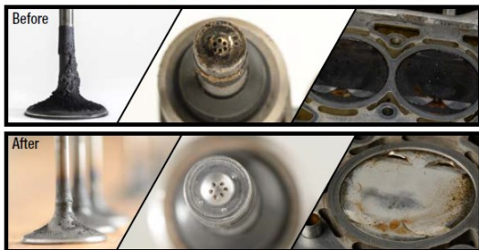
Intake Valve, Fuel Injector and Piston Head at 39,035 miles
