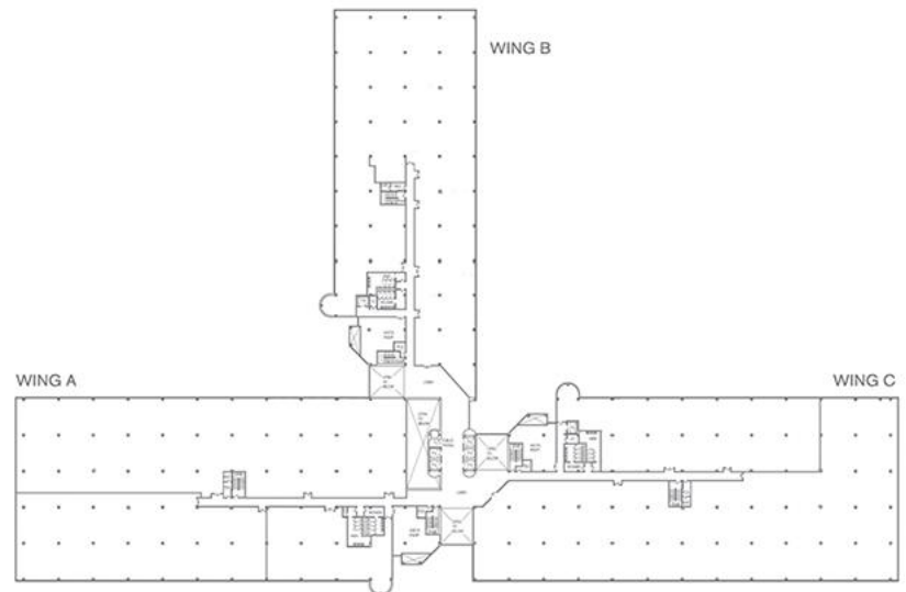
Typical Floor Plate
